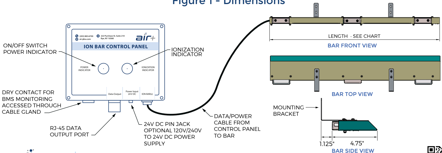
Figure 1 - Dimensions
