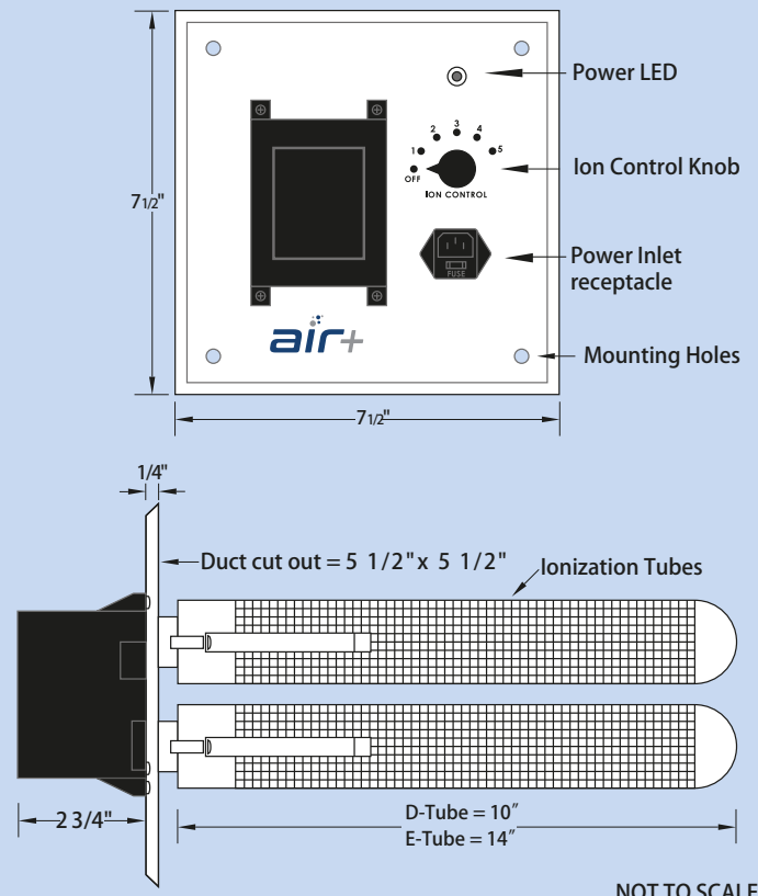
FIGURE 2: DIMENSIONS
