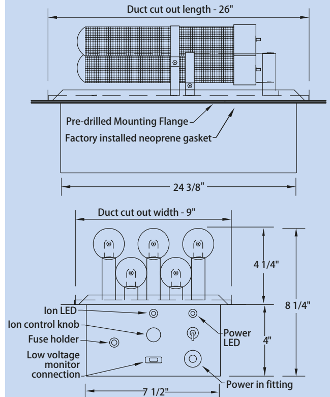
FIGURE 2: DIMENSIONS
